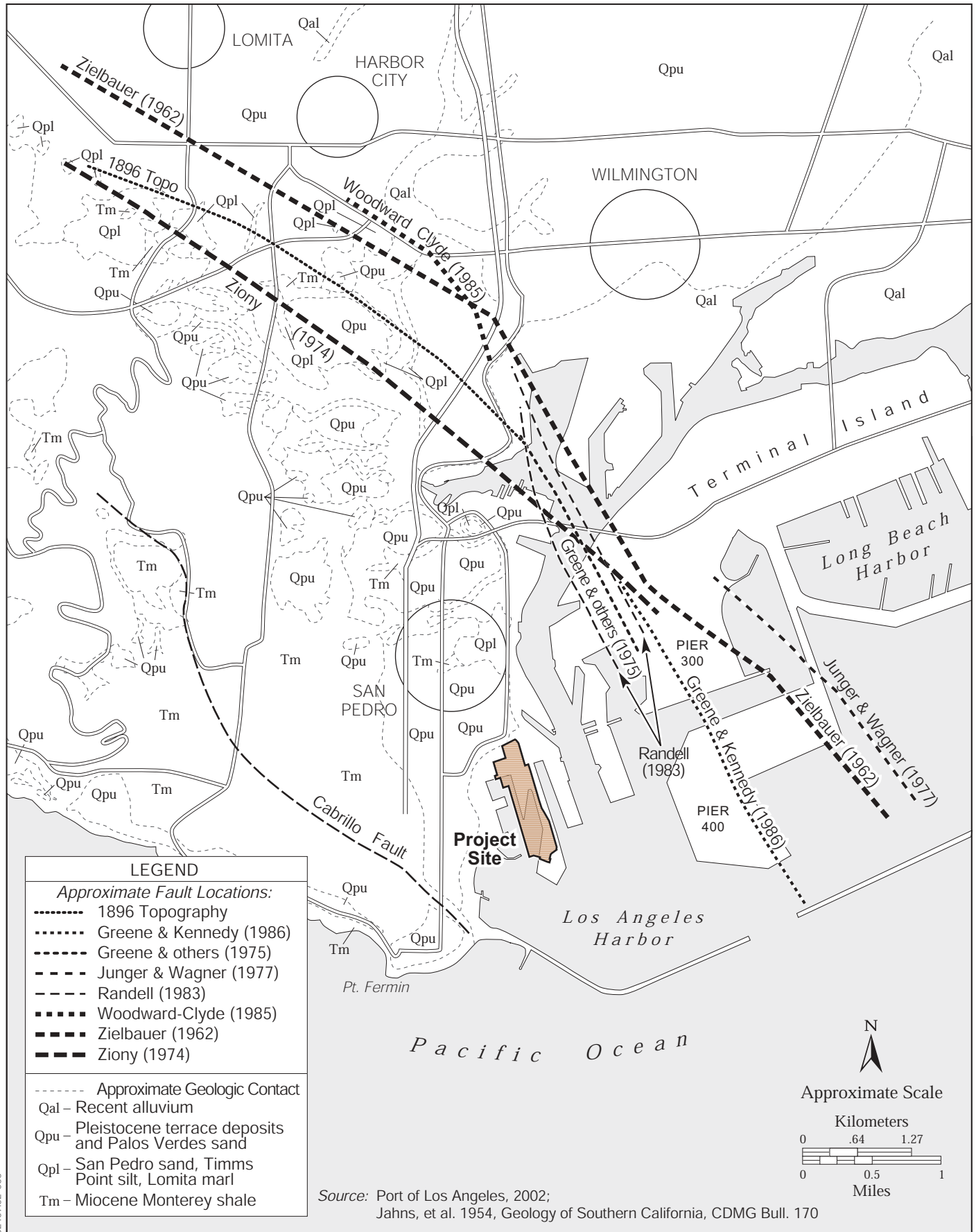
Figure 3.7-2 Palos Verdes Fault Zone
