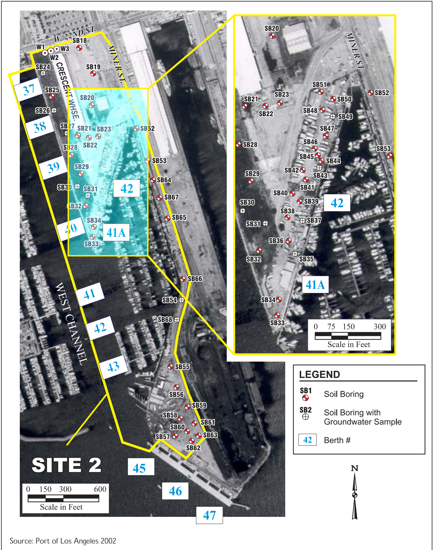
Figure 3.8-2b Soil Boring/Groundwater Sample Locations
